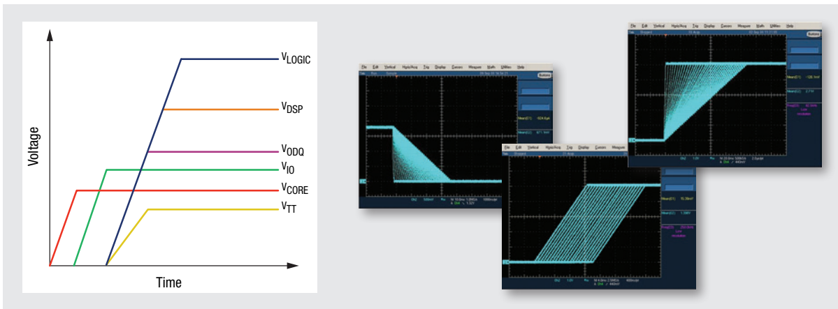
Control Power Up/Down Sequencing with Different Delays and Slopes using PowerArchitect™
